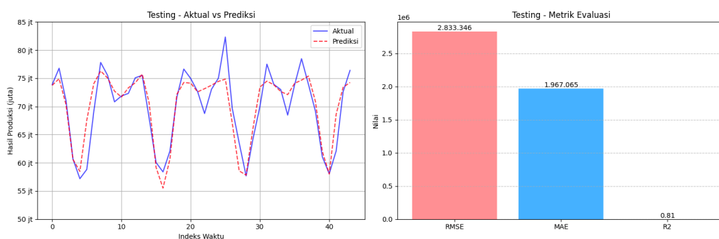
(a) Data Prediksi vs Aktual Testing
