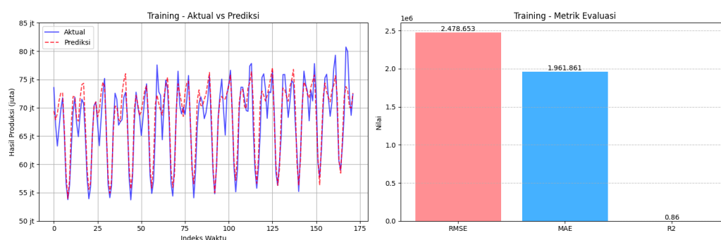
(a) Data Prediksi vs Aktual Training
