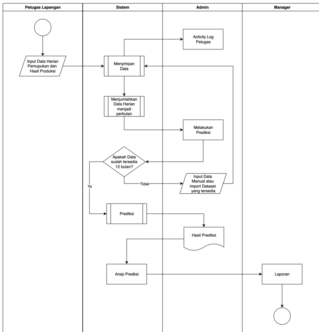
Gambar 3. 9 Flowchart Sistem
