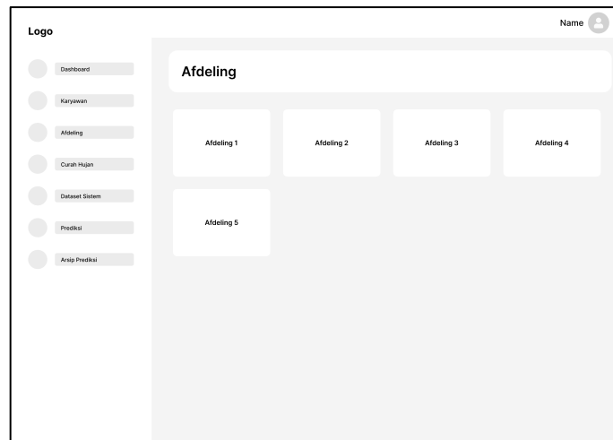
Gambar 3. 16 Interface Afdeling
